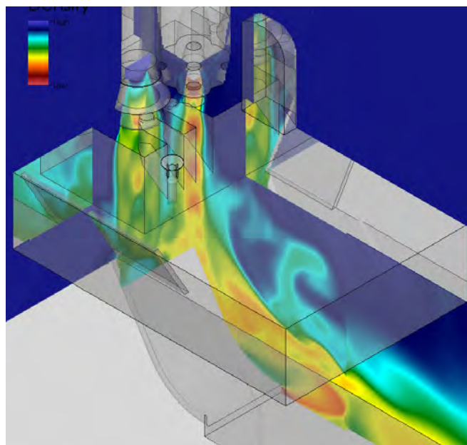
High-fidelity CFD simulation of launch environment conditions for an early candidate heavy-lift launch vehicle and design. (Cetin Kiris, Jeffrey Housman, Michael Barad, NASA/Ames)
