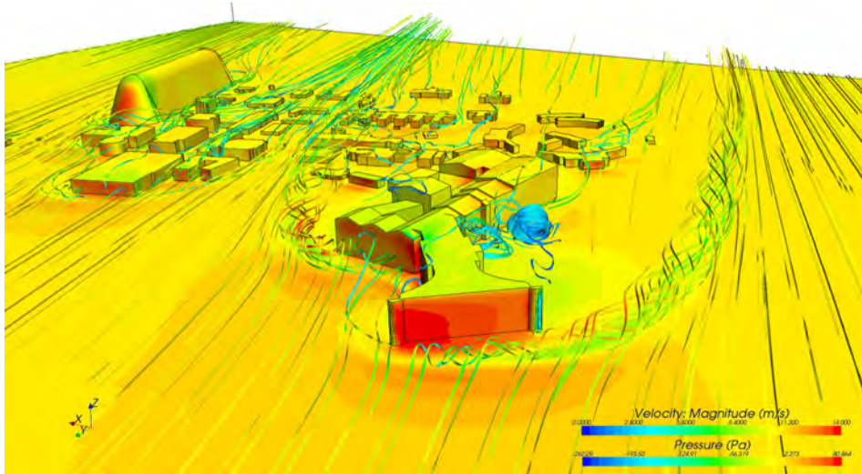
Large-scale CFD simulation of wind flows around the Sustainability Base green building at NASA Ames Research Center. (Michael Barad, NASA/Ames)
