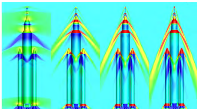
CFD simulations of ascent aerodynamics for an early candidate crew launch vehicle design. (Michael Barad, NASA Ames)
